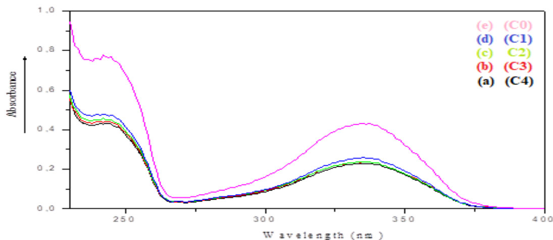
Fig. 7: Absorption spectra of ATB with various concentration of \beta -CD.
