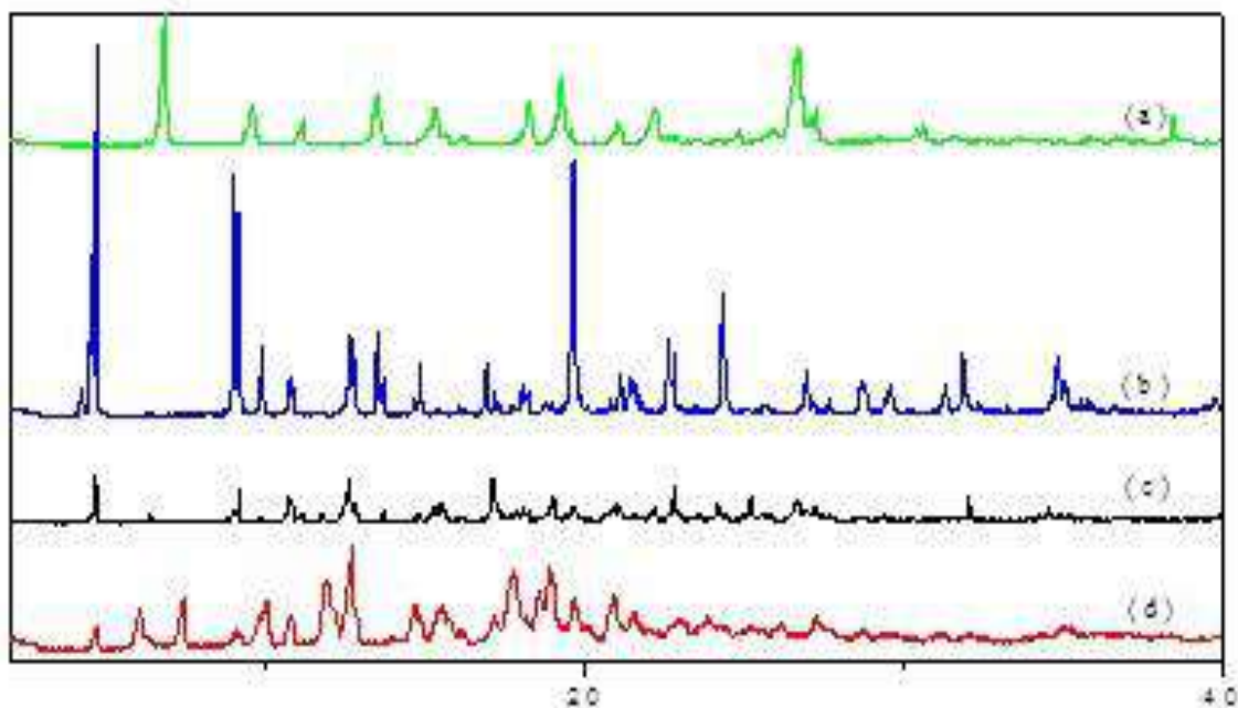
Fig. 3: Powder X-ray diffractometry of (a) ATB; (b) cyclodextrin; (c) physical mixture with molar ratio 1:1 (guest:host) and (d) inclusion compound.
