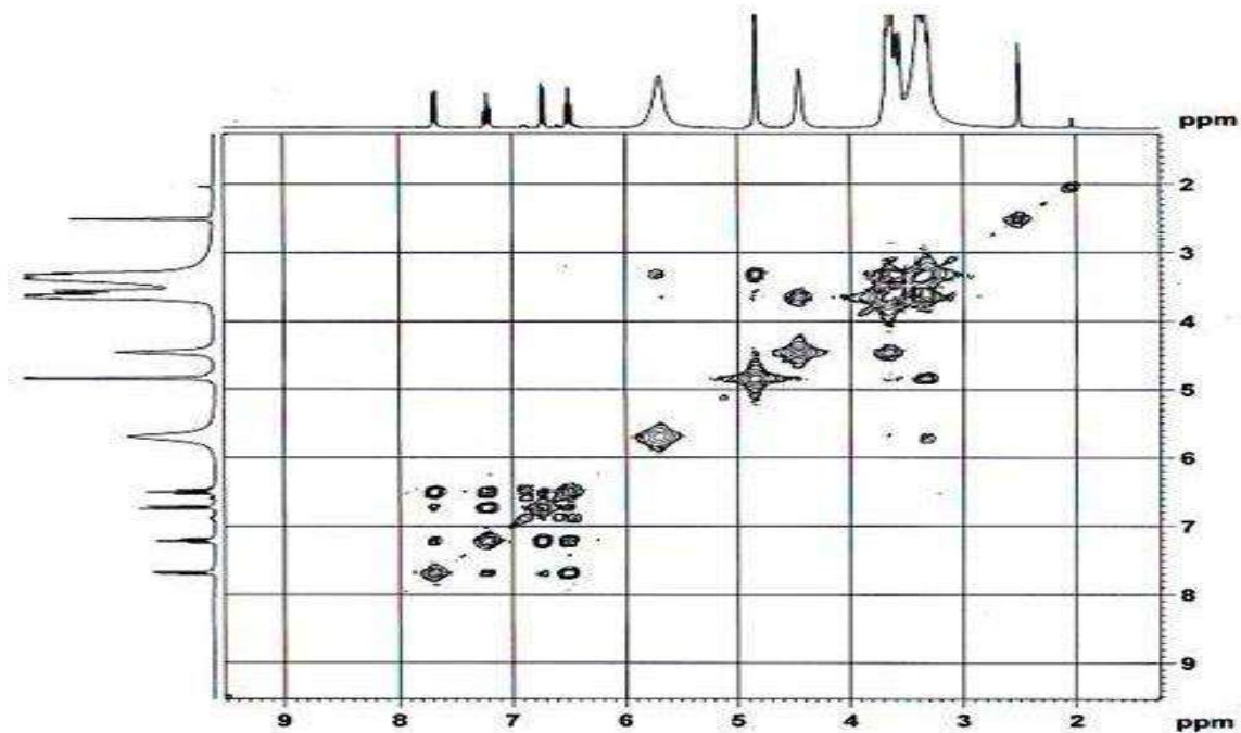
Fig. 5: NMR Noesy of inclusion compound \beta CD/ ATB.
