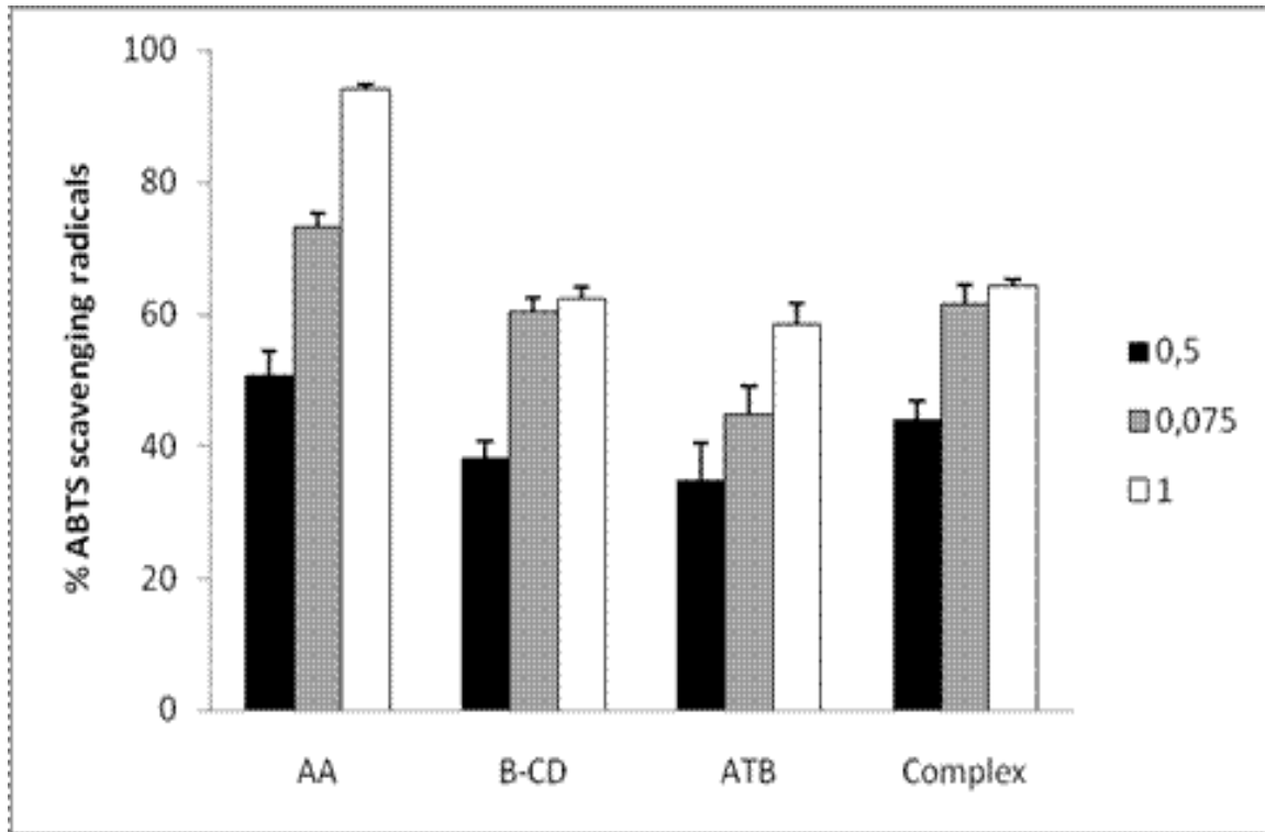
Fig. 10 ABTS radical scavenging ability: tested compounds (B-CD; ATB and Complex); AA: ascorbic acid).
