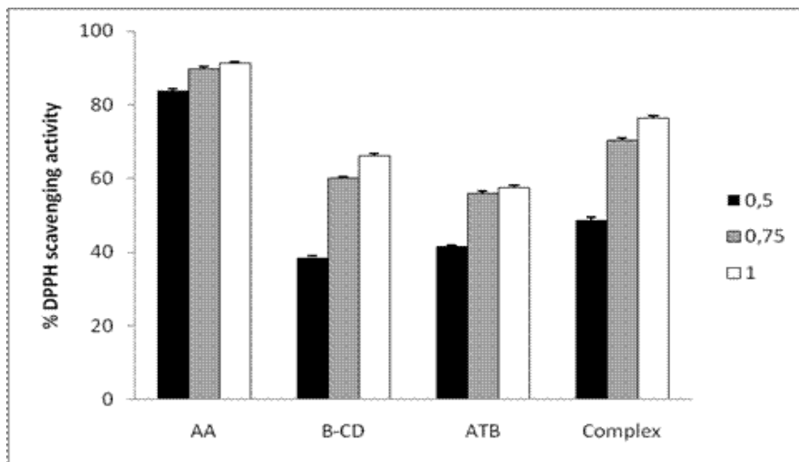
Fig. 9 DPPH Radical Scavenging Activity: tested compounds (B-CD; ATB and Complex); AA: ascorbic acid.
