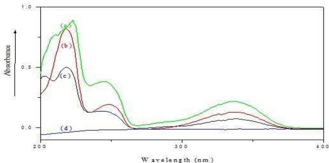
Fig. 4: UV spectra of (a) ATB; (b): physical mixture in molar ratio 1:1(guest:host); (c): inclusion compound and (d): cyclodextrin.
