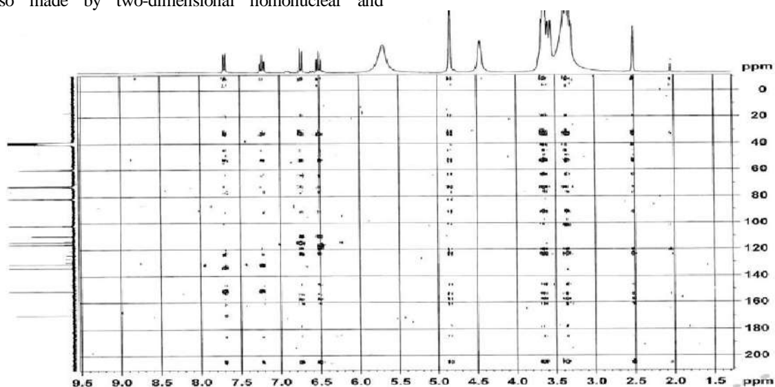
Fig. 6: HMBC spectra of inclusion compound \beta -CD/ ATB.
