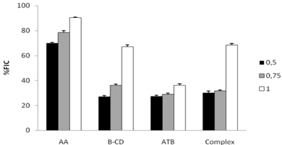
Fig. 13 Ferrous ion chelating (FIC) ability: tested compounds (B-CD; ATB and Complex); AA: ascorbic acid).
