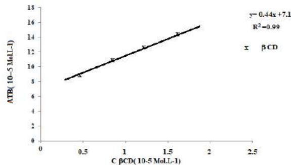
Fig. 8: Phase solubility diagram of ATB in aqueous solution of Beta CD.
