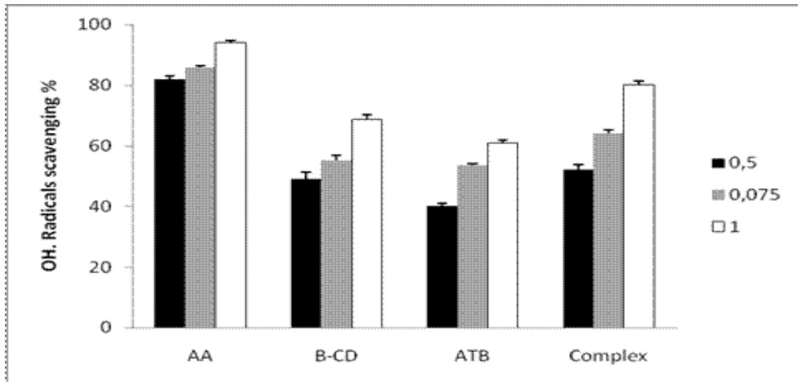
Fig. 11: OH radical scavenging ability: tested compounds (B-CD; ATB and Complex); AA: ascorbic acid).
