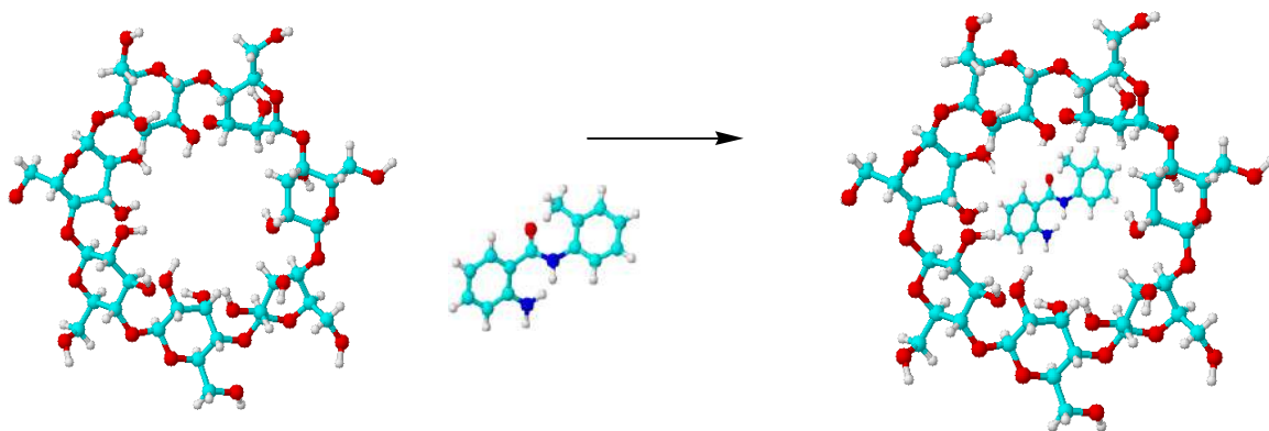
Fig. 2: Synthesis of inclusion compound of ATB and \beta -CD.
