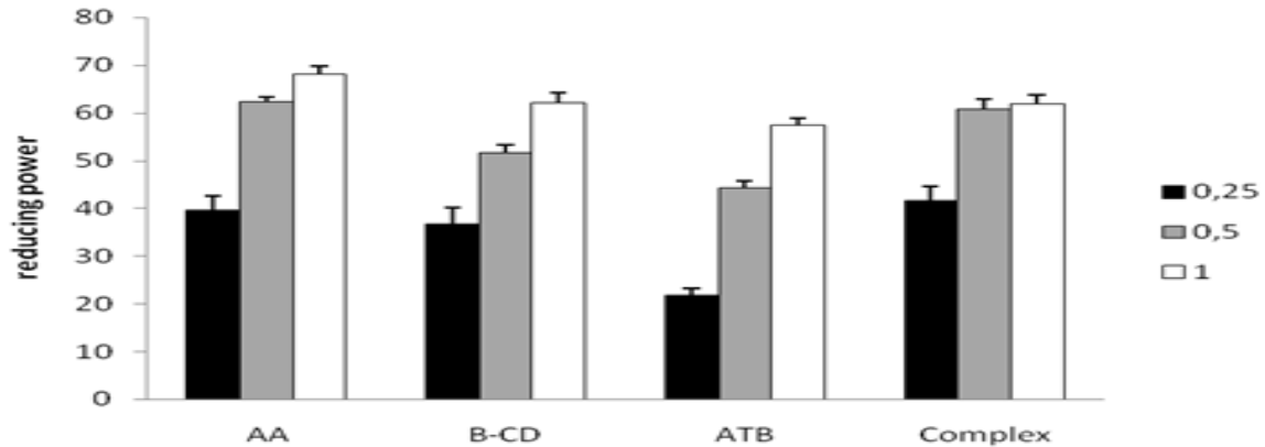
Fig. 12: Reducing power assay: tested compounds (B-CD; ATB and Complex); AA: ascorbic acid
